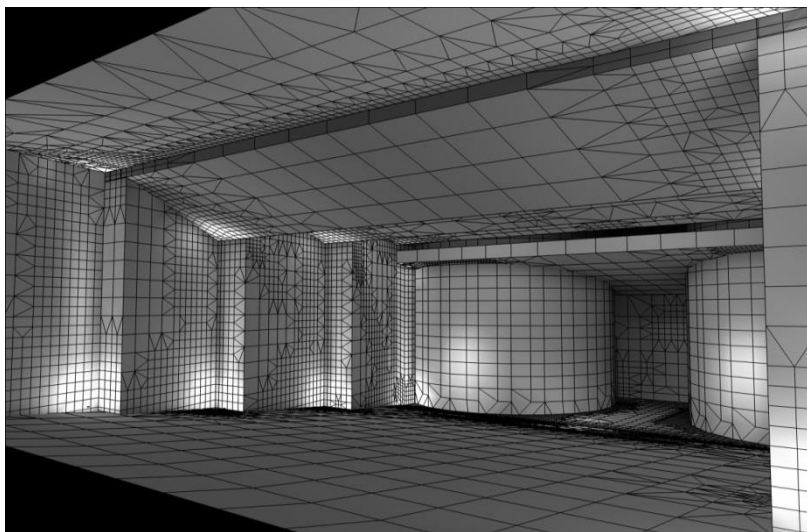
AGi32 created architectural geometry
